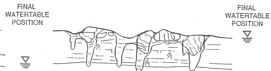
T-6 CONTINUED DISSOLUTION LOWERS RELIEF AND CAUSE SPIRES AND COLUMNS TO COLLAPSE. PASSIVE AND DISPLACIVE HALITE CEMENTS DEVELOP AND SUBAQUEOUS HALITE DEPOSITION OCCURS IN TOPOGRAPHIC LOWS AS THE WATERTABLE MOVES HIGHER.
