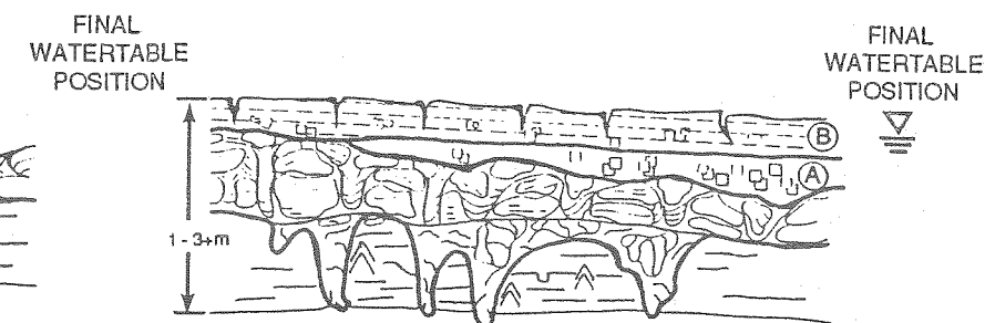
T-12 (A) MIXED HALITE AND MUD ARE DEPOSITED SUBAQUEOUSLY AND REWORKED BY SOLUTION AND PRECIPITATION OF DISPLACIVE CEMENTS DURING MINOR WATERTABLE FLUCTUATIONS. (B) MUD IS DEPOSITED AND REWORKED BY PRECIPITATION AND DISSOLUTION OF DISPLACIVE HALITE CEMENTS.
