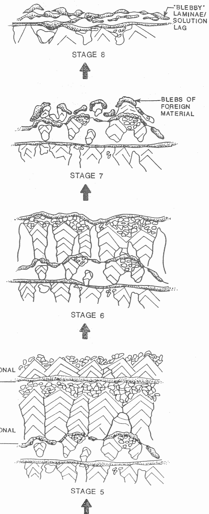
FIGURE 20 DEVELOPMENT OF SMALL-SCALE SALADO HALITE FABRICS.
