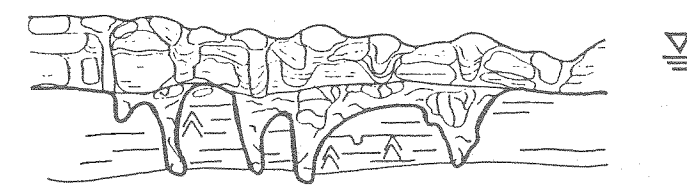
T-11 COLLAPSE OF HIGH RELIEF FEATURES FOLLOWS CONTINUED DISSOLUTION. PASSIVE AND DISPLACIVE HALITE CEMENTS DEVELOP AND SUBAQUEOUS HALITE DEPOSITION OCCURS AS THE WATERTABLE MOVES HIGHER.
