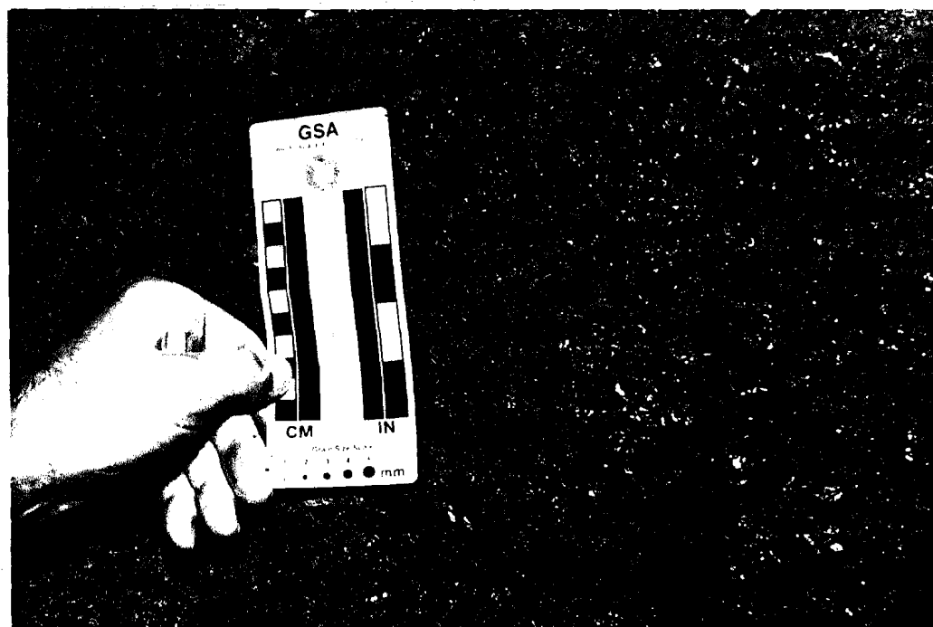
Figure 19 Halitic mudstone lithofacies with isolated displacive halite crystals.
