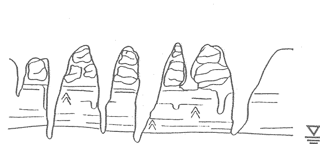
T-5 FOLLOWING A LARGE WATERTABLE DROP, DISSOLUTION CREATES SPIRES AND COLUMNS.
