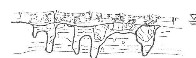
T-7 HALITE ACCUMULATES UNDER SUBAQUEOUS CONDITIONS AND IS THEN REWORKED FOLLOWING WATERTABLE DROPS.
